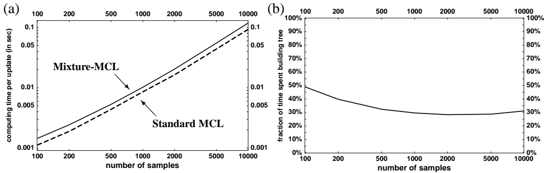
Fig. 21. (a) Time (in seconds on a 500MHz Pentium PC) required for one full belief computation using regular MCL (dashed line) and Mixture-MCL (solid line), plotted as a function of the number of particles. (b) Percentage of time spent generating density trees in Mixture-MCL. All results are averaged over 1,000 updates using the robot simulator.
