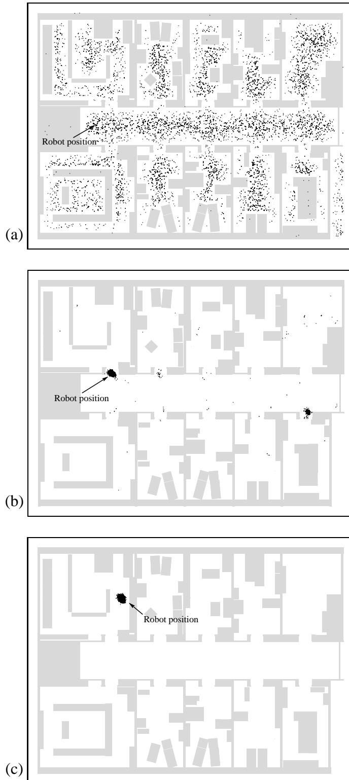
Fig. 6. Global localization of a mobile robot using MCL (10,000 samples): (a) initial particle set, uniformly distributed (projected into 2D). (b) Particles after approximately 2 meters of robot motion. Due to environment symmetry, most particles are centered around two locations. (c) Particle set after moving into a room, thereby breaking the symmetry. These experiments were carried out with a RWI B21 robot.
