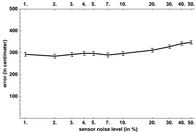
Fig. 12. Error of dual MCL as a function of the sensor noise. The error appears to increase monotonically with the sensor noise, but the overall error level is high. Compare this graph to Figure 10. These results were obtained through simulation.
