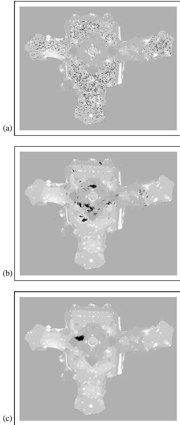
Fig. 9. Global localization of a mobile robot using a camera pointed at the ceiling. This experiment has been carried out with the Minerva tour-guide robot, a RWI B18 robot.
