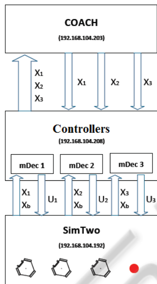
Figure 5: Communications between applications diagram.
