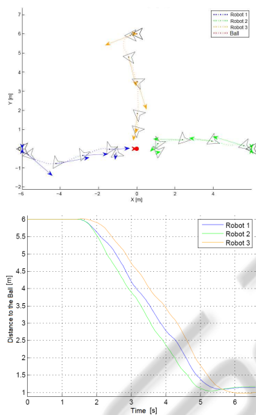
Figure 6: Convergence into formation, simulation 1.
