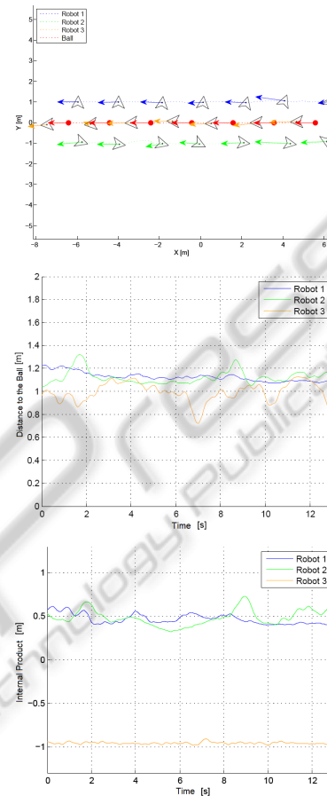
Figure 10: Maintaining formation in a straight line, simulation 1b.
