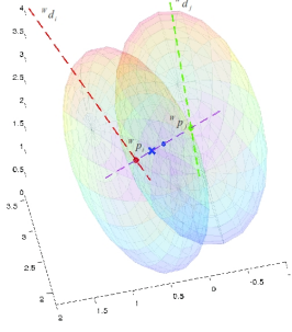
Fig. 4. Snapshot from the covariance 3D ellipse of P_{int_i} and P_{int_j} and the intersection point obtained from the algorithm. Mid-Point Triangulation method (blue dot). Triangulation based on the state covariance value (blue cross). Perpendicular vector W_{d_c} to (W_{d_i}, W_{d_j}) (purple line).
