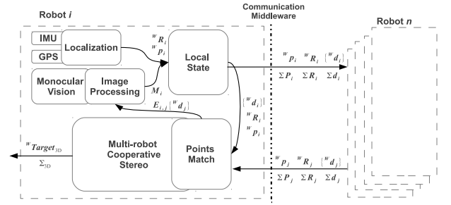
Fig. 2. Multi-Robot Cooperative Stereo Architecture
